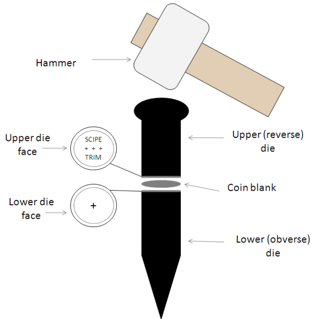
Figure 3.1 Schematic illustration of how a coin is made using a hammer. The die faces are engraved with the design and a coin blank is placed between them. The dies are then held together whilst struck with a heavy hammer. The lower (obverse) die has a spike so it can be secured into a work station, which was normally a wooden block, before coins were struck.
